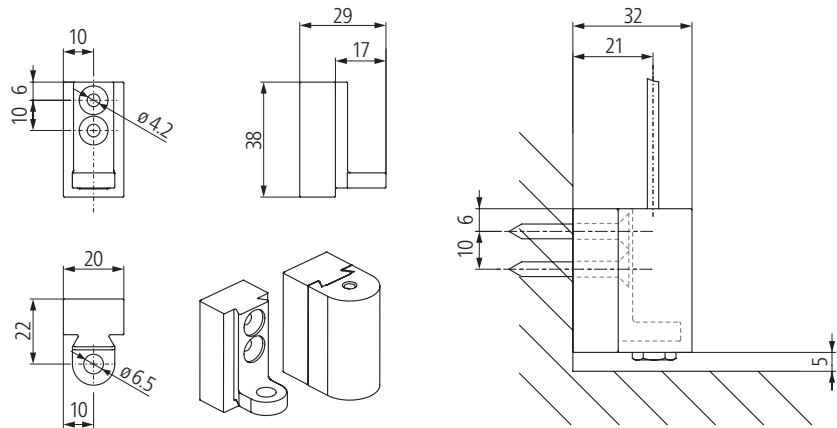
VertiTex 38 x 20 x 32 mm standard rope holder
