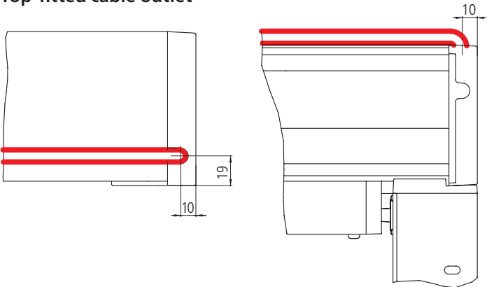
Top-fitted cable outlet
