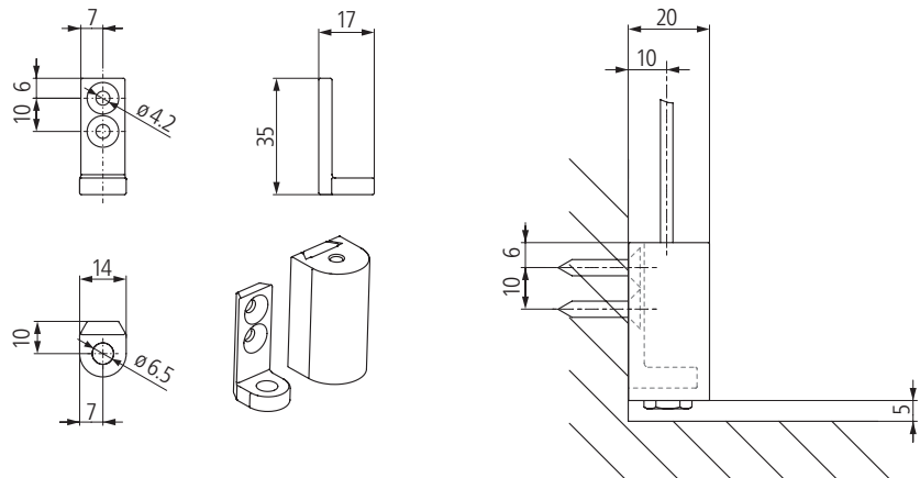
VertiTex 38 x 20 x 20 mm rope holder
