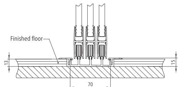
Flat floor rail trimmed in, on both sides with floor gap sealing profile
