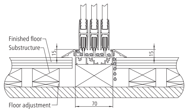
Floor rail with CleanCase® partly trimmed in with threshold profile
