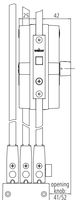
Lockcase and hung bolt with opening knob
