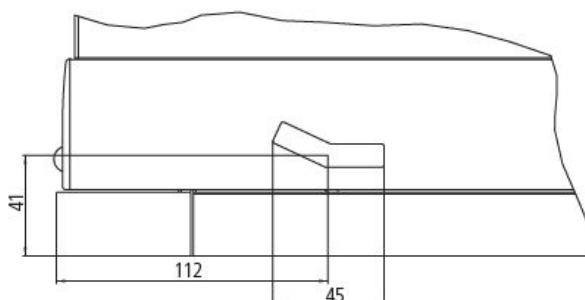
Detail of floor rail with leaf profile with locking lever
