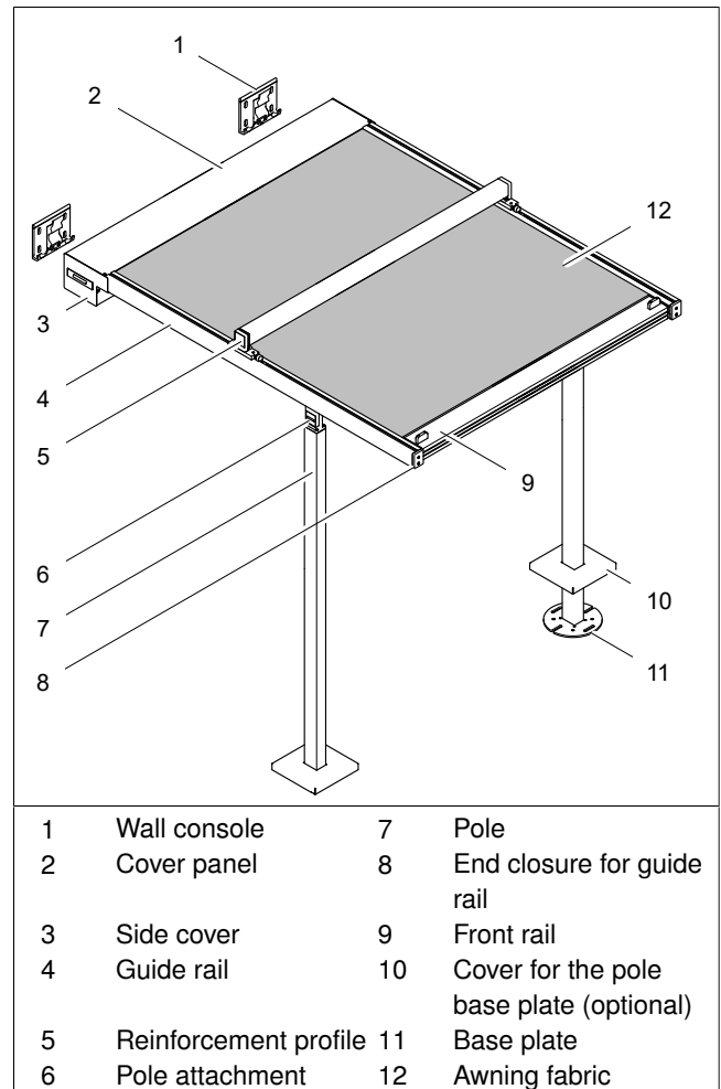
Fig. 1: Parts overview of pergola awning Perea P20
