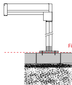
Post attachment on concrete floor slabs or foundations
