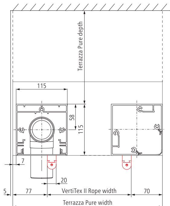
VertiTex II Rope in front with lateral wall
