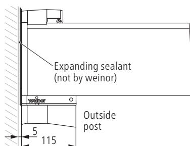
Gutter and post position on a partial side wall – wall offset 5 mm
