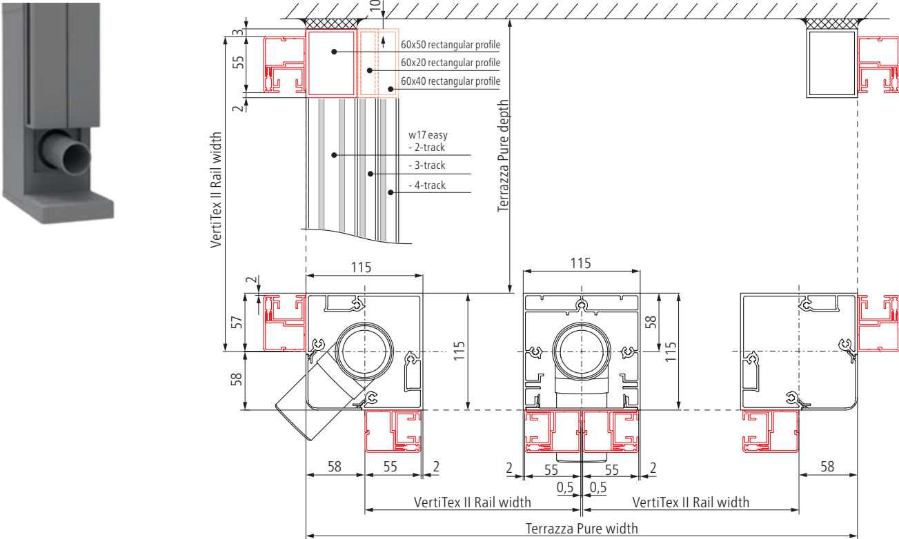
VertiTex II Rail/Zip multi-section unit in front
