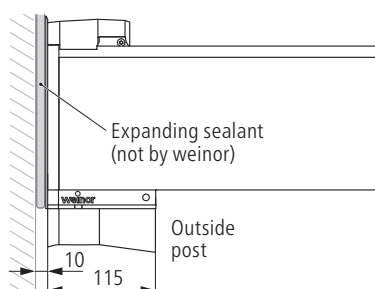
Gutter and post position on a partial side wall – wall offset 10 mm
