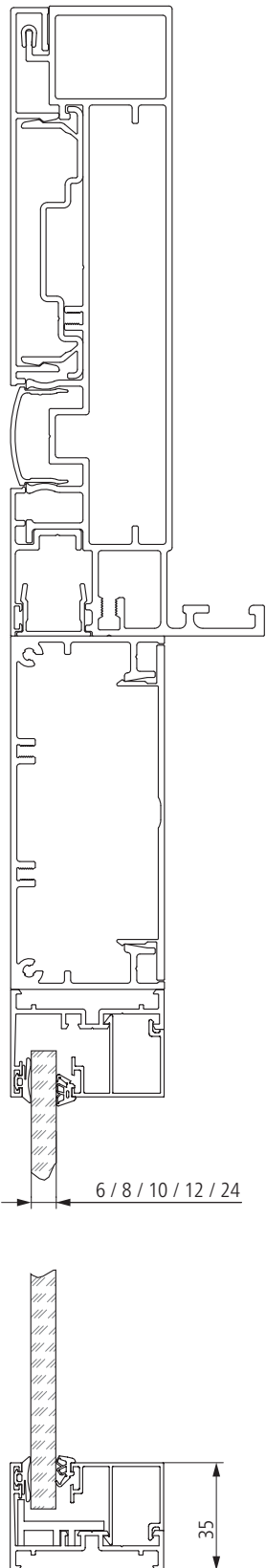
Side roof support with 115 x 50 mm frame widener (for retrofitting) and w50-c SUPER LITE 35 fixed glazing
