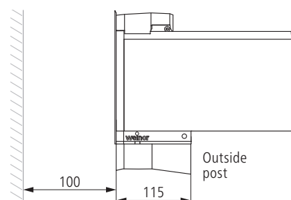
Gutter and post position on a partial side wall – wall offset 100 mm
