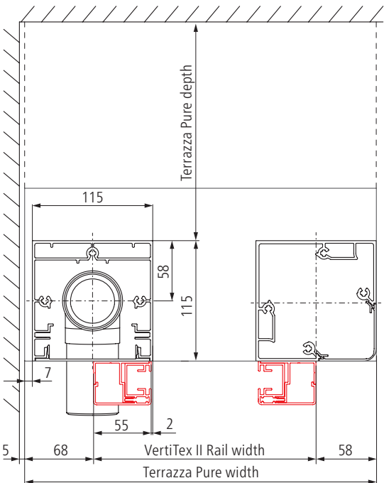
VertiTex II Rail/Zip in front with lateral wall
