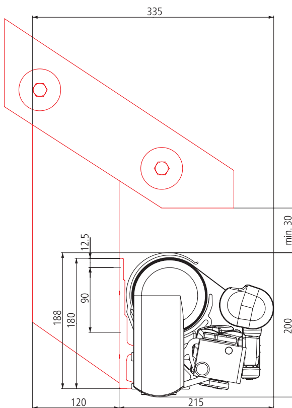
Side view of rafter installation with roofless Topas
