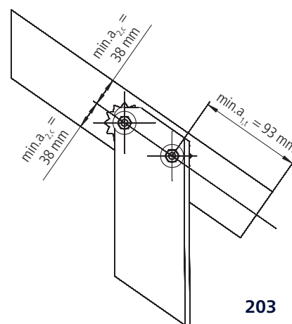
Rafter bracket without mounting plate
