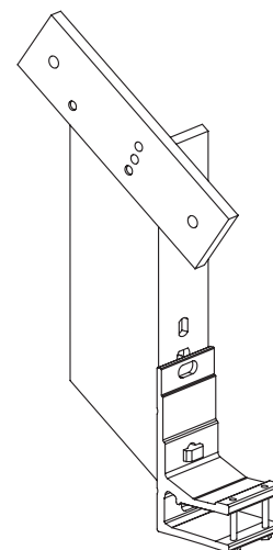
Rafter bracket with mounting plate weinor recommends using mounting plates for rafter brackets.
