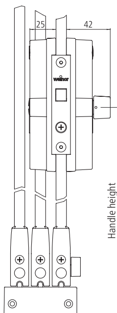
Knob for lockcase and hung bolt
