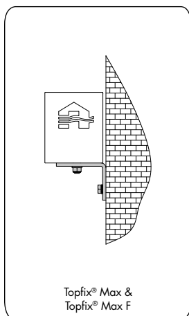
Wall fastening of the side channels
