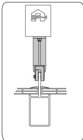
Fixing the assembly feet to a T-mullion (glass below)
