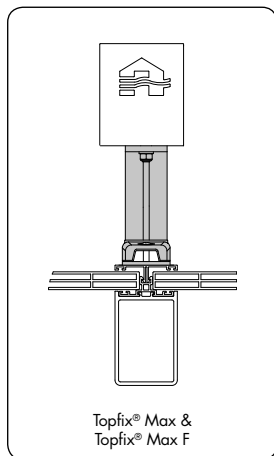
Fixing the assembly feet to a mullion (glass above)
