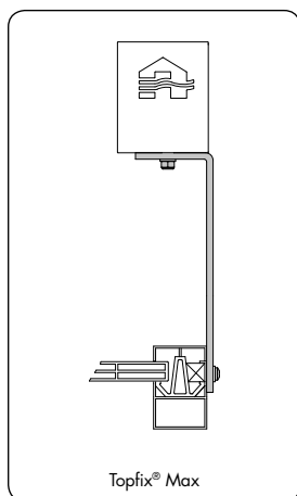
Fixing the side channels on the sides of the conservatory
