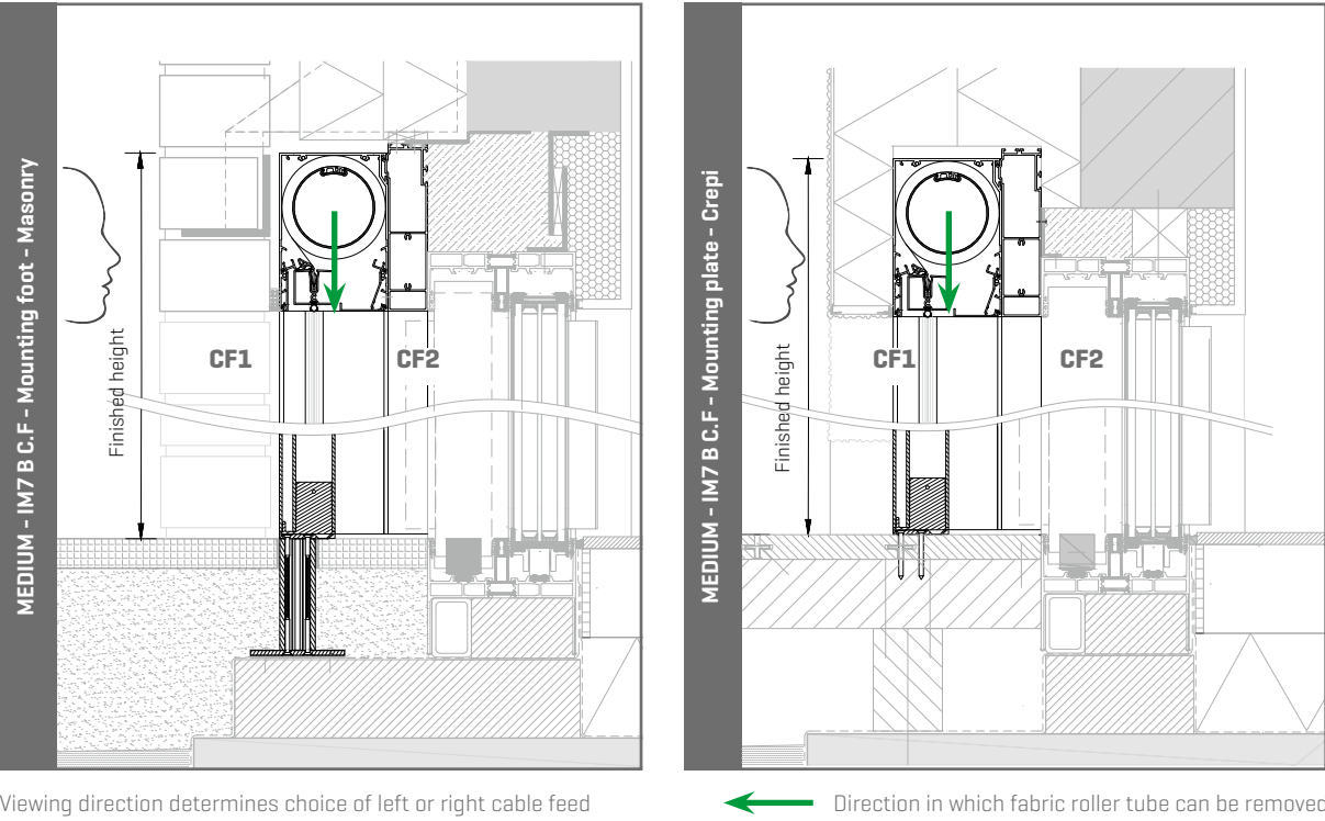
Viewing direction determines choice of left or right cable feed Direction in which fabric roller tube can be removed
