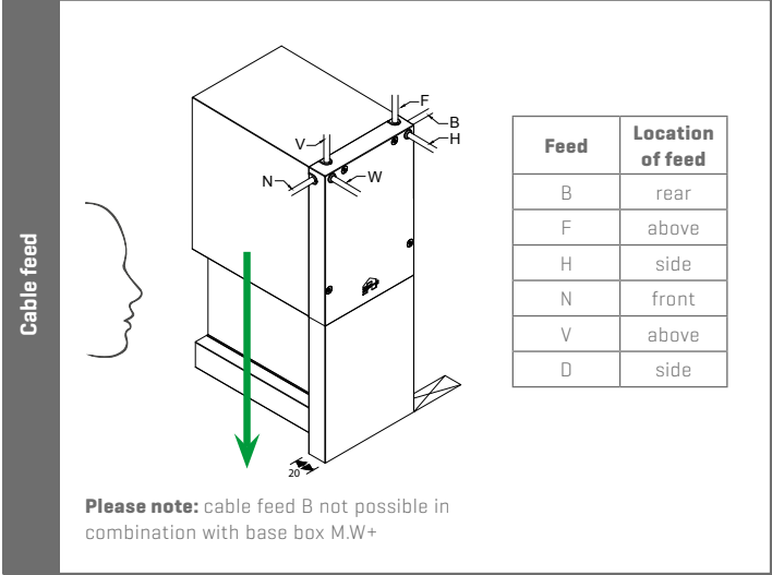
Viewing direction determines choice of left or right cable feed
