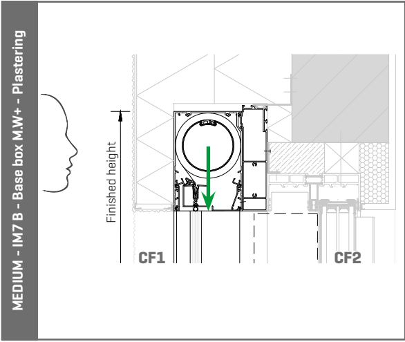
Direction in which fabric roller tube can be removed
