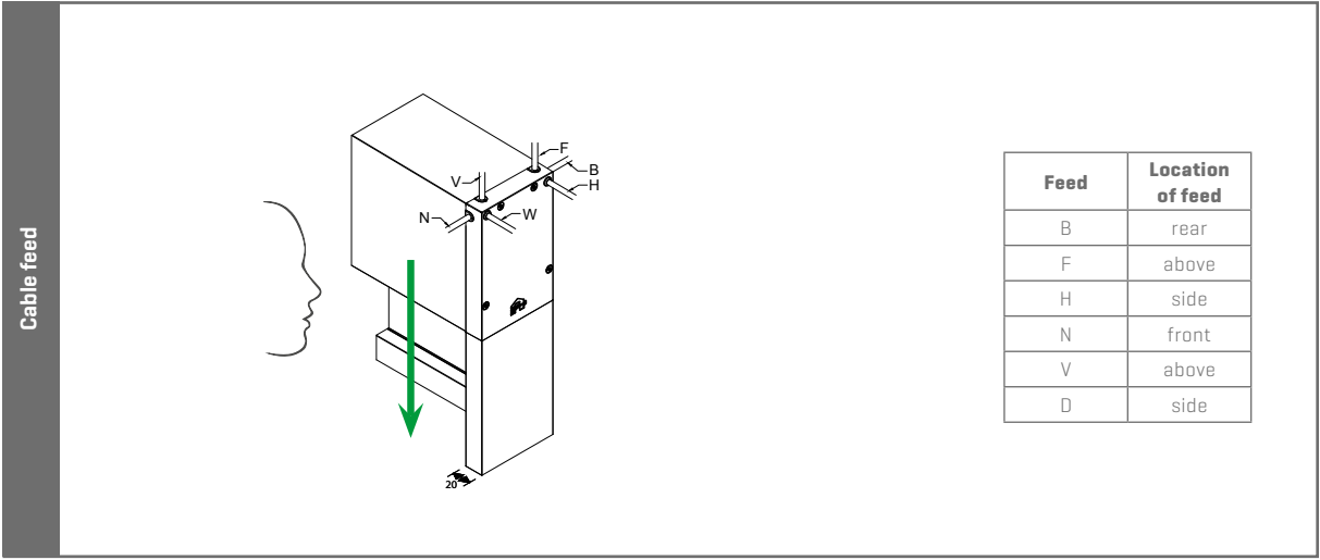
Viewing direction determines choice of left or right cable feed
