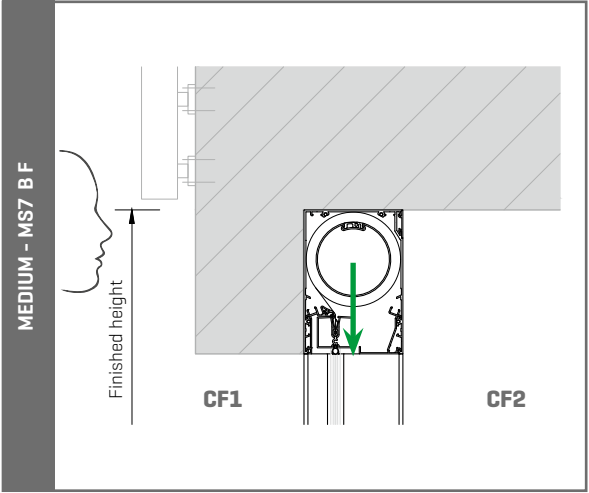
Direction in which fabric roller tube can be removed
