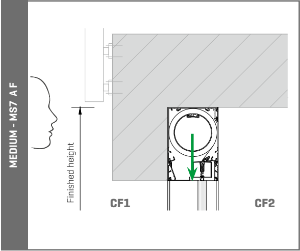
Viewing direction determines choice of left or right cable feed
